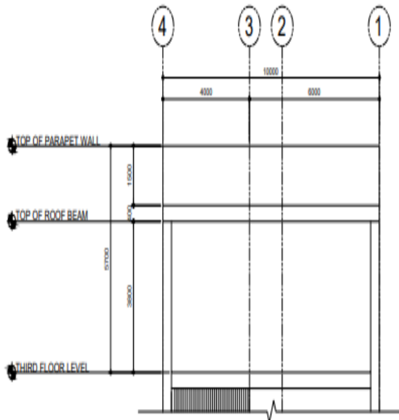
2 REAR ELEVATION A-3 SCALE 1:100
