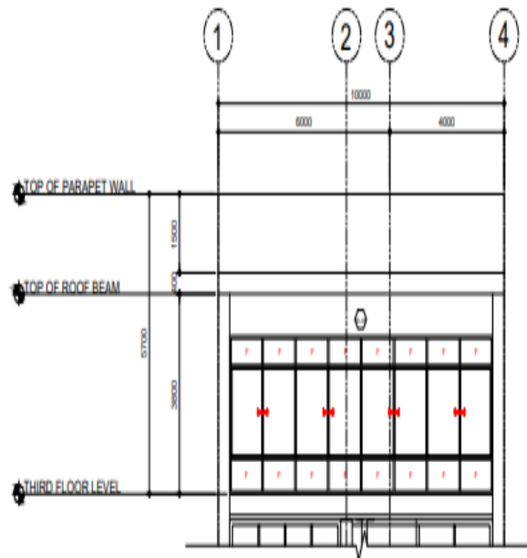
1 FRONT ELEVATION A-3 SCALE 1:100
