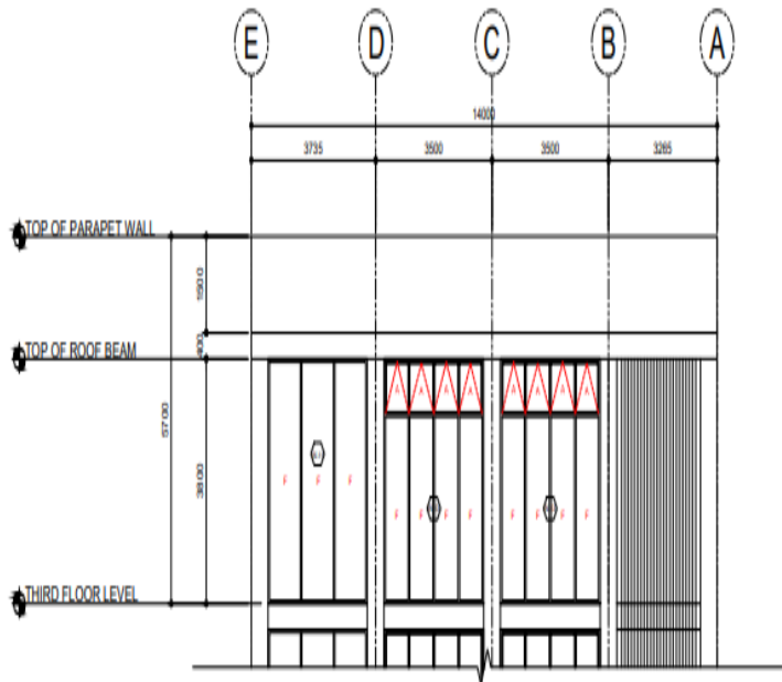
2 LEFT SIDE ELEVATION SCALE 1:100
