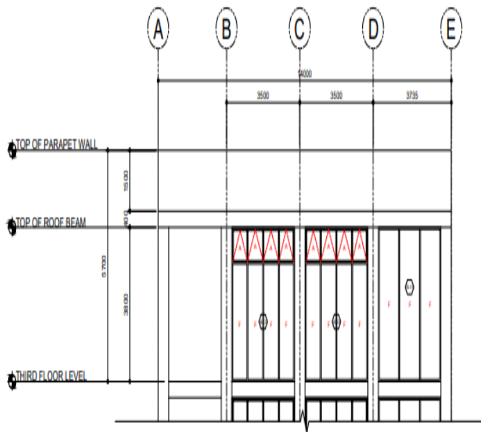
1 RIGHT SIDE ELEVATION SCALE 1:100
